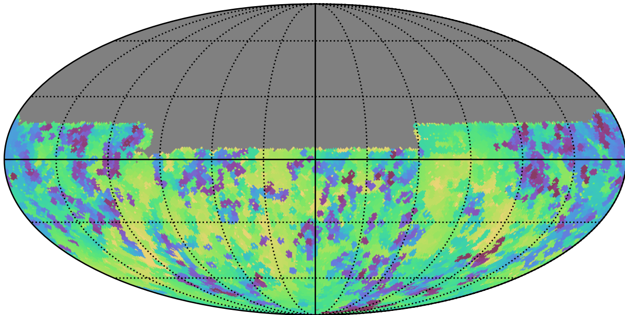
scp_reweight_v3.3_10yrs Yr 1 y band: Min skyBrightness
