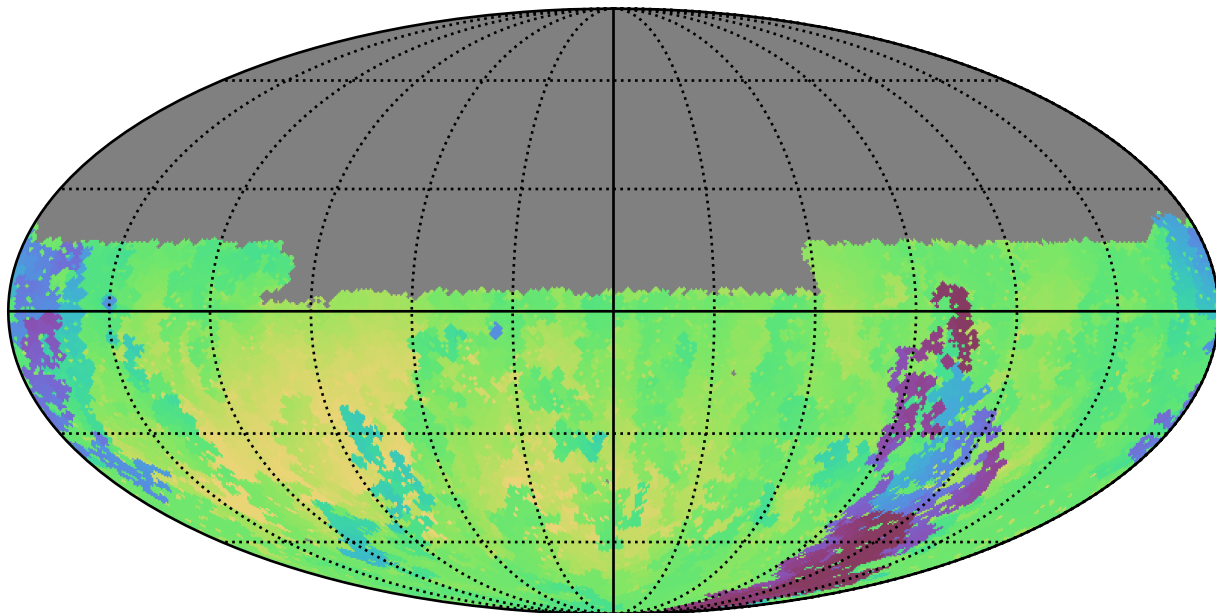
scp_reweight_v3.3_10yrs Yr 1 u band: Min skyBrightness
