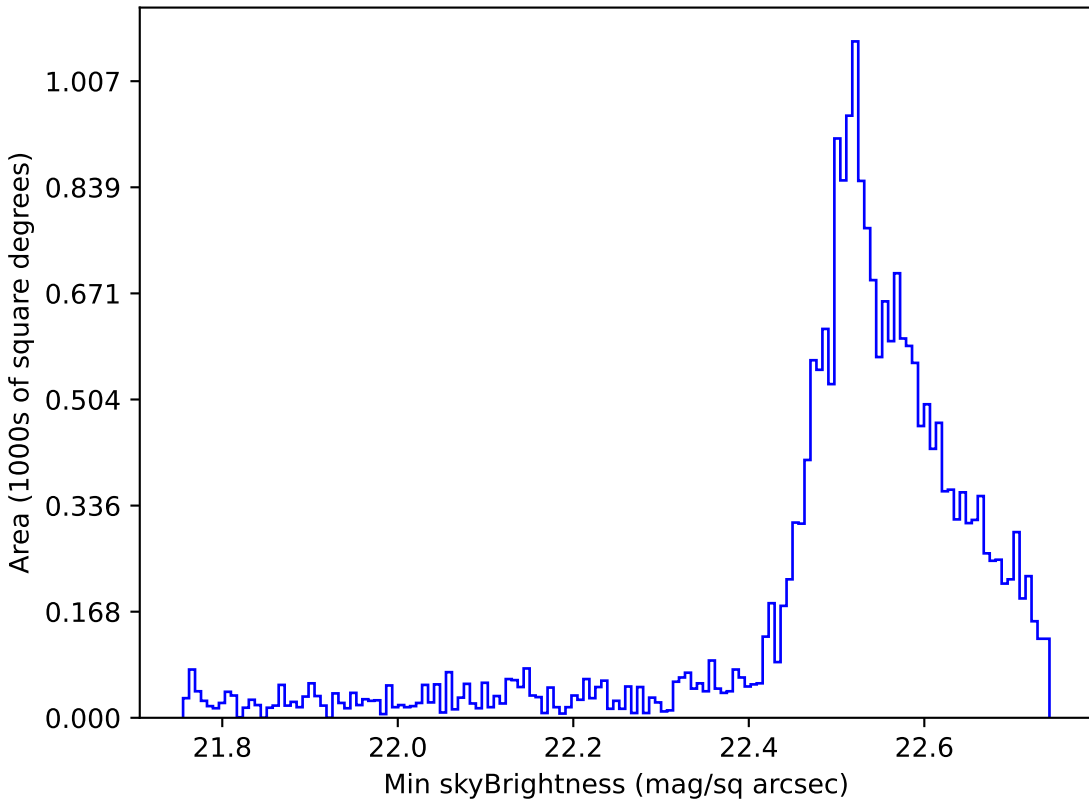
scp_reweight_v3.3_10yrs Yr 1 u band: Min skyBrightness
