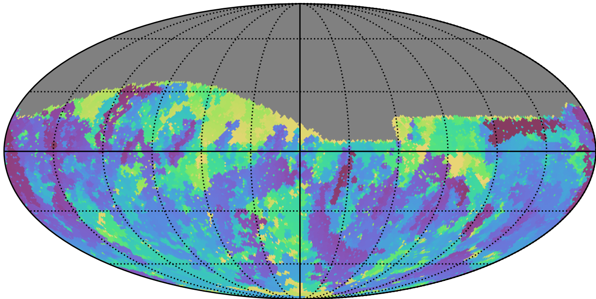
scp_reweight_v3.3_10yrs Yr 1 r band: Min skyBrightness
