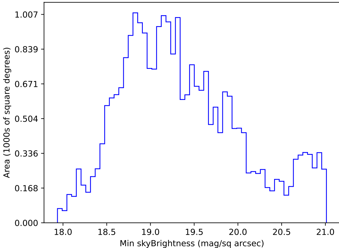
scp_reweight_v3.3_10yrs Yr 1 r band: Min skyBrightness
