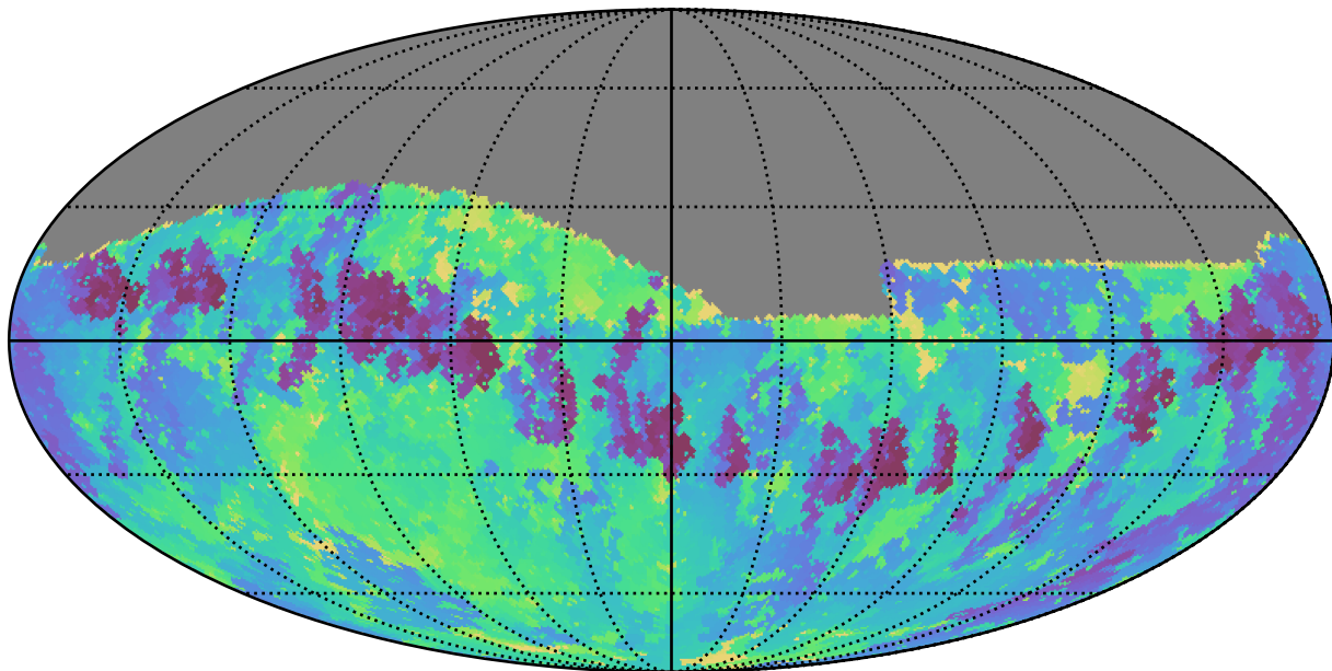
scp_reweight_v3.3_10yrs Yr 1 i band: Min skyBrightness
