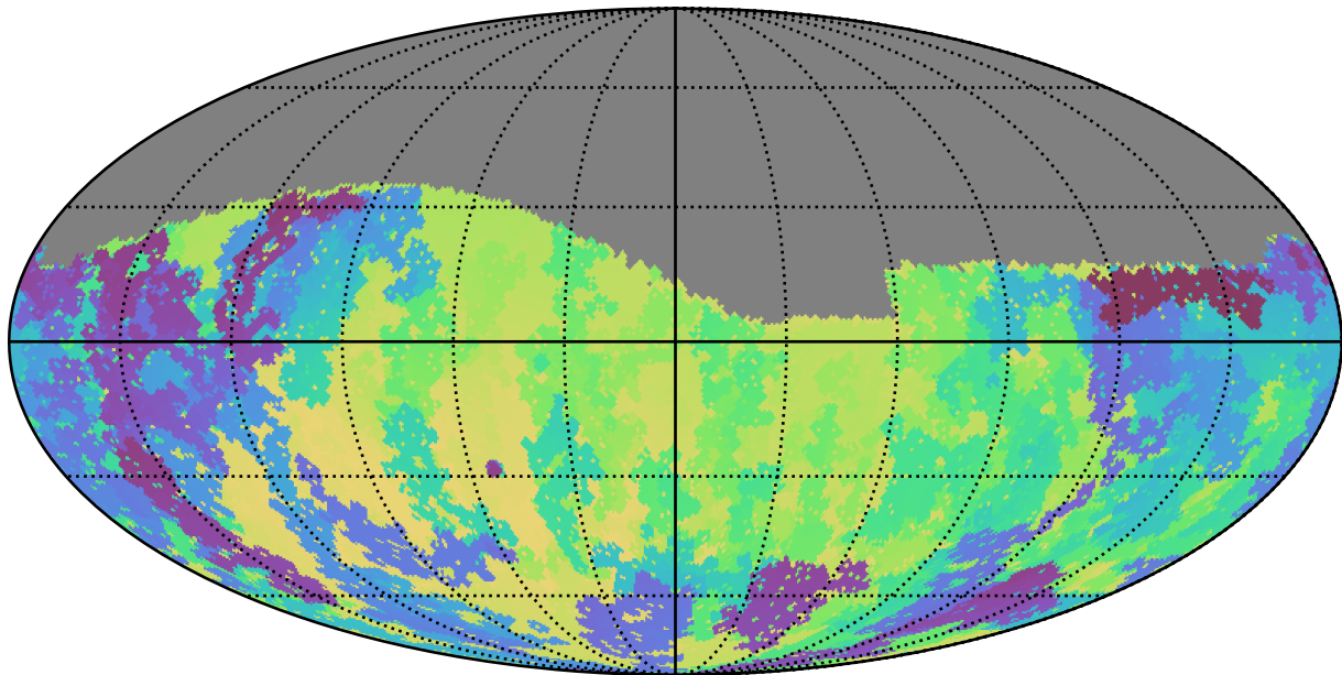
scp_reweight_v3.3_10yrs Yr 1 g band: Min skyBrightness
