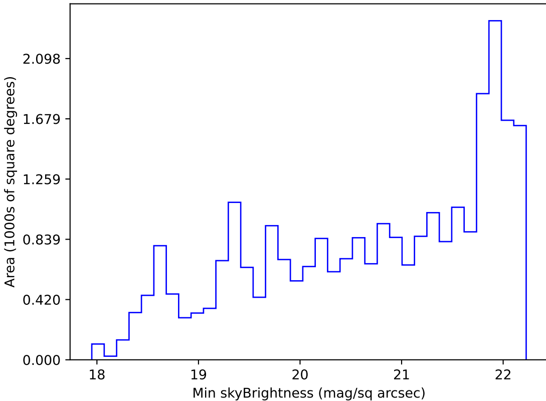
scp_reweight_v3.3_10yrs Yr 1 g band: Min skyBrightness
