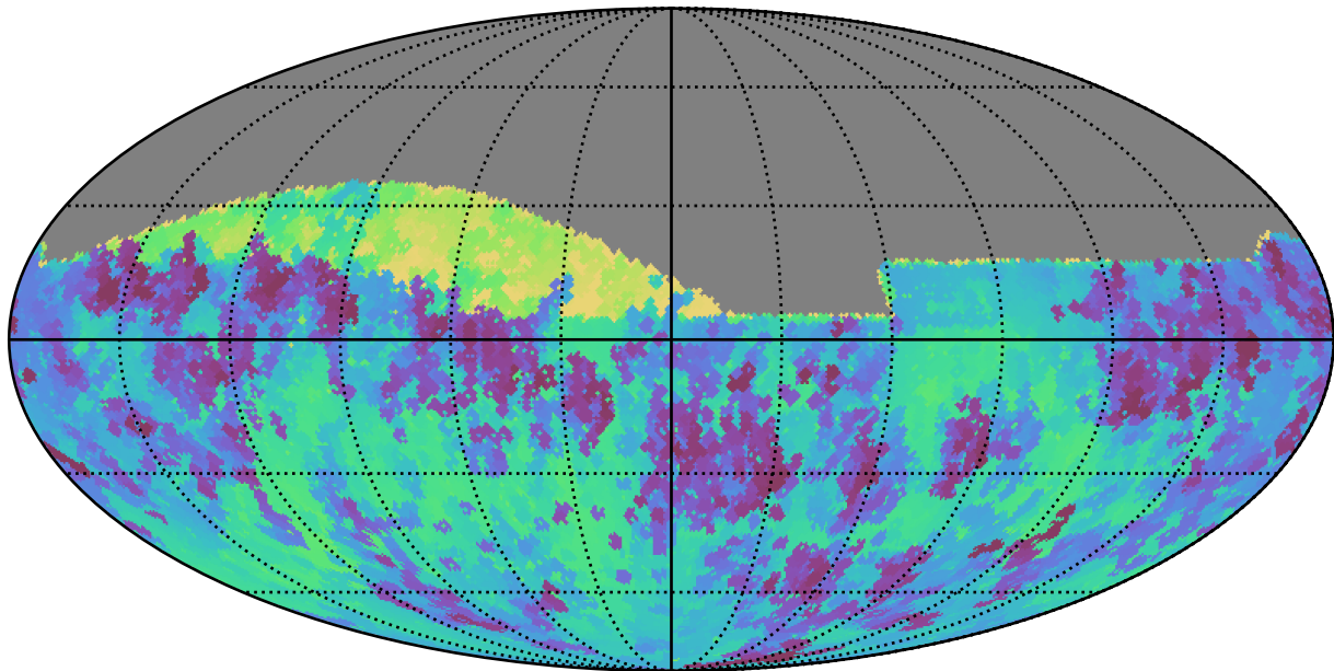
scp_reweight_v3.3_10yrs Yr 1 all bands: Min skyBrightness
