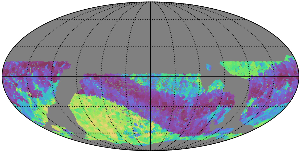
scp_reweight_v3.3_10yrs WFD z band: Min skyBrightness
