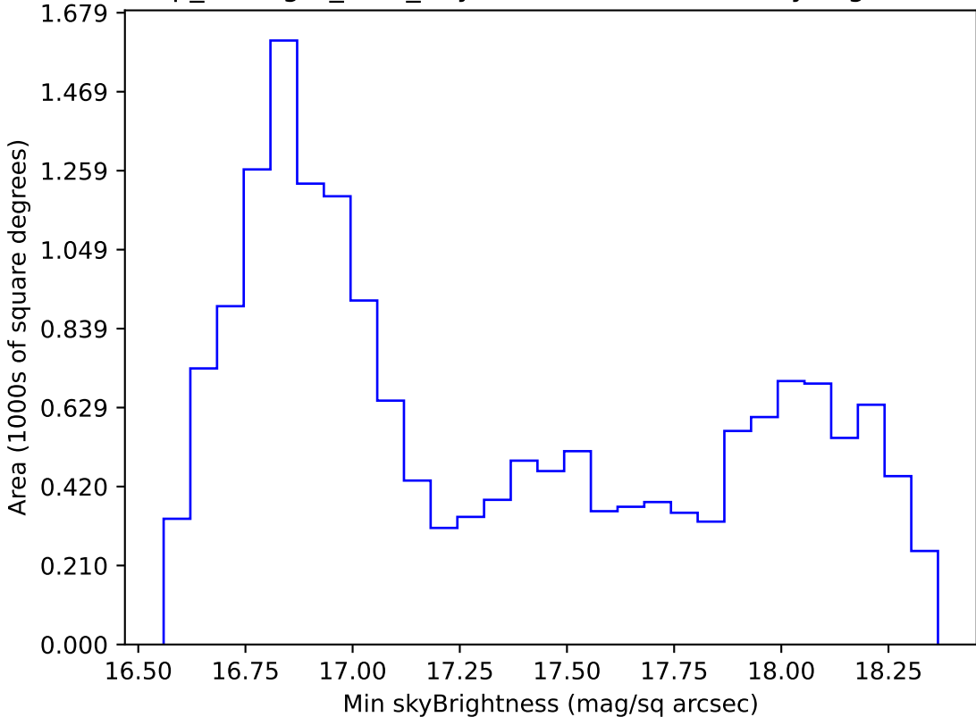
scp_reweight_v3.3_10yrs WFD z band: Min skyBrightness
