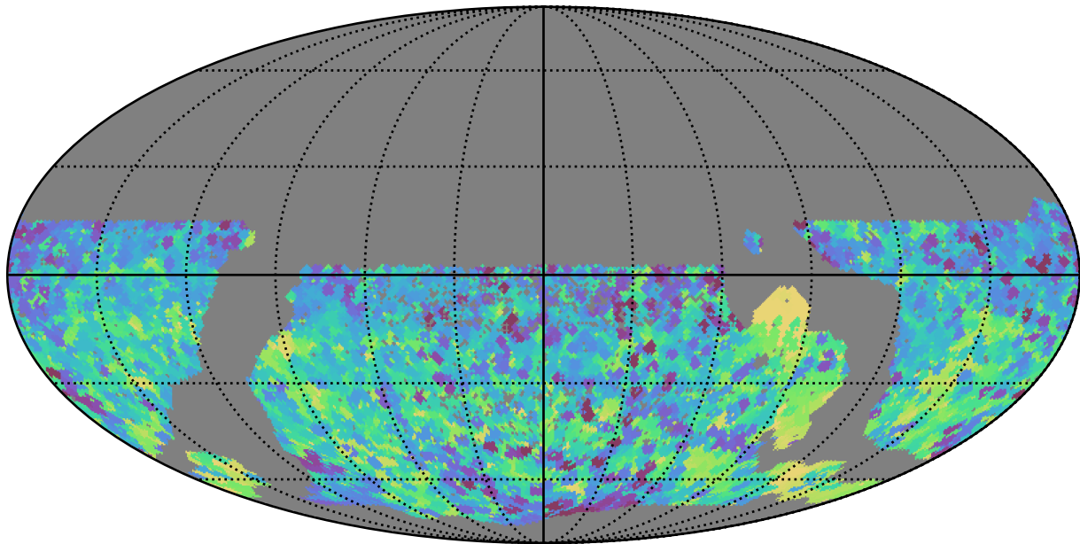
scp_reweight_v3.3_10yrs WFD y band: Min skyBrightness
