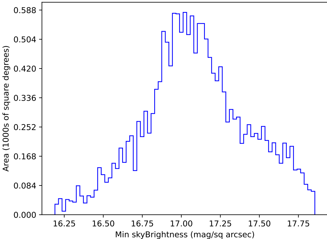
scp_reweight_v3.3_10yrs WFD y band: Min skyBrightness
