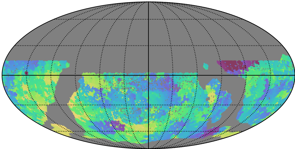
scp_reweight_v3.3_10yrs WFD u band: Min skyBrightness
