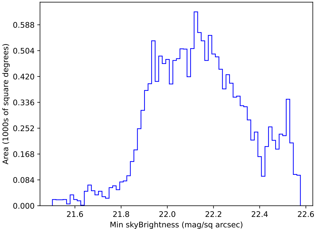
scp_reweight_v3.3_10yrs WFD u band: Min skyBrightness
