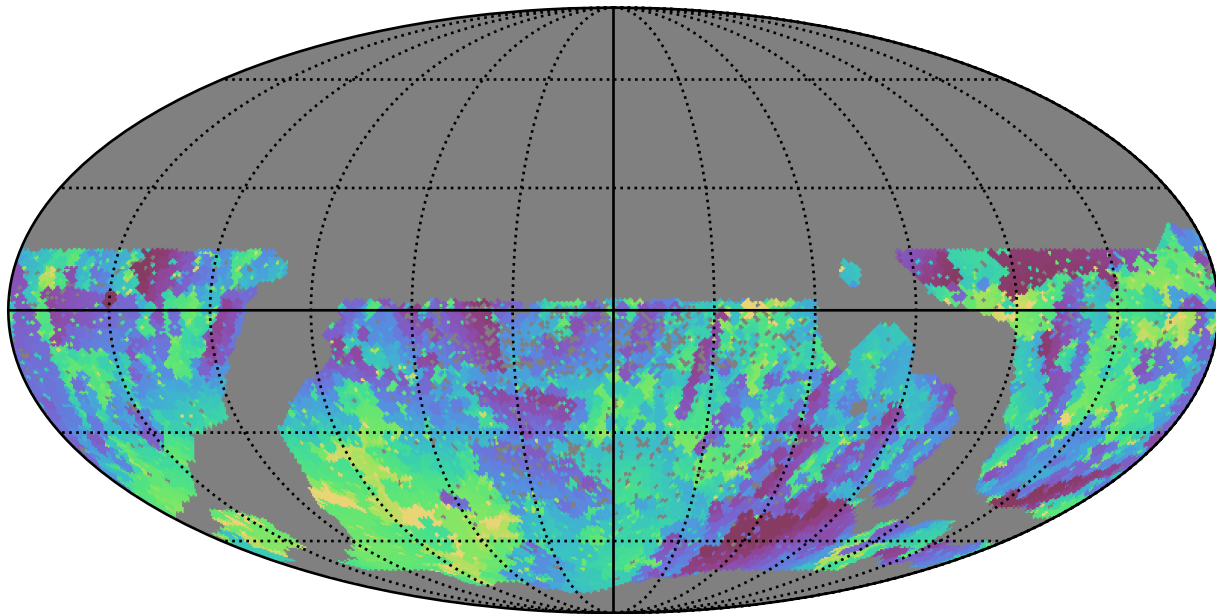
scp_reweight_v3.3_10yrs WFD r band: Min skyBrightness
