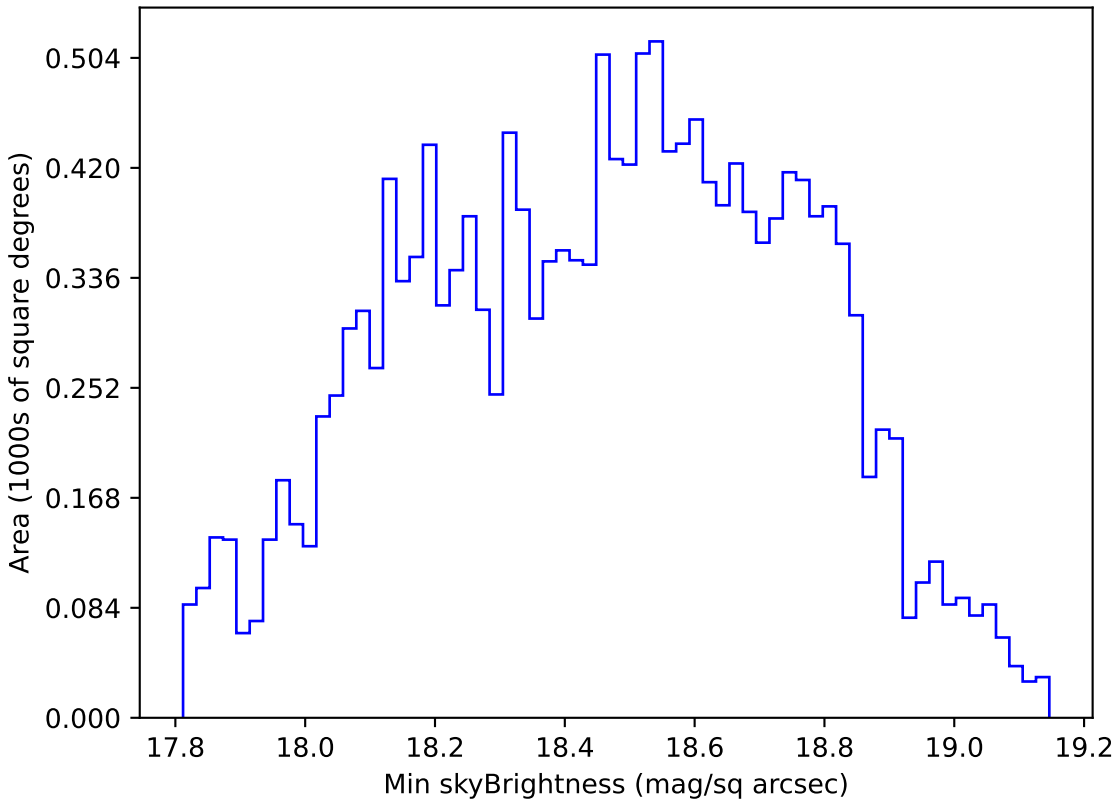
scp_reweight_v3.3_10yrs WFD r band: Min skyBrightness
