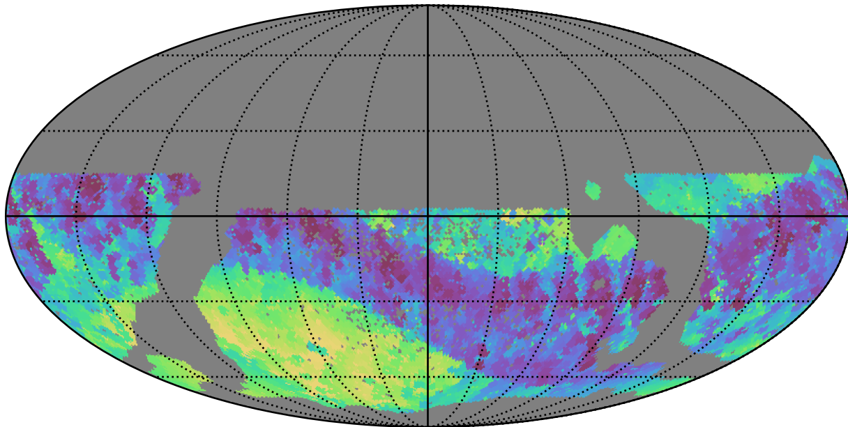
scp_reweight_v3.3_10yrs WFD i band: Min skyBrightness
