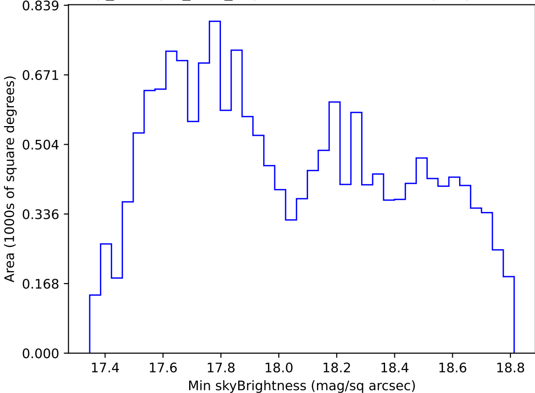
scp_reweight_v3.3_10yrs WFD i band: Min skyBrightness
