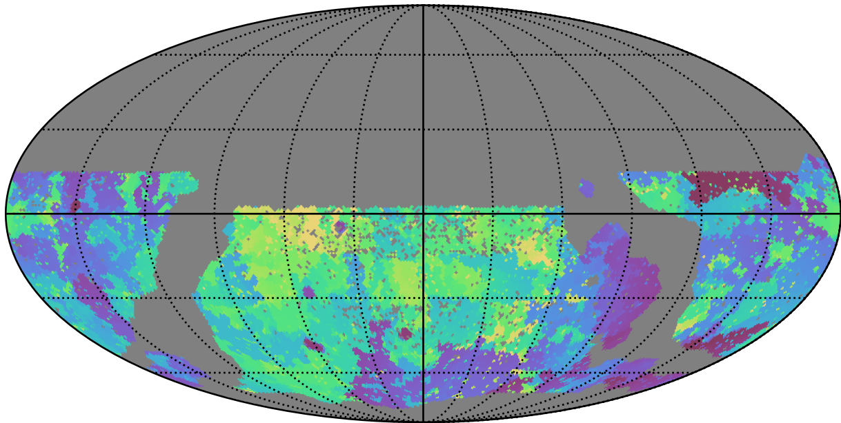
scp_reweight_v3.3_10yrs WFD g band: Min skyBrightness
