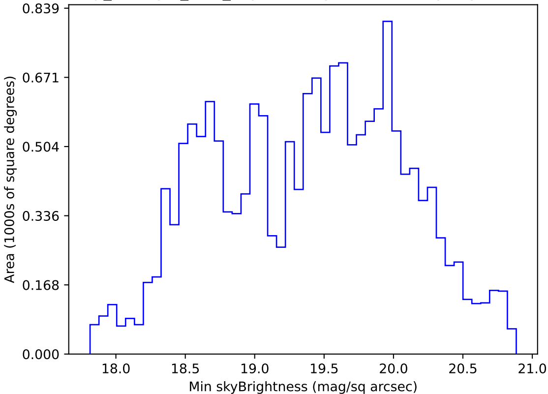
scp_reweight_v3.3_10yrs WFD g band: Min skyBrightness
