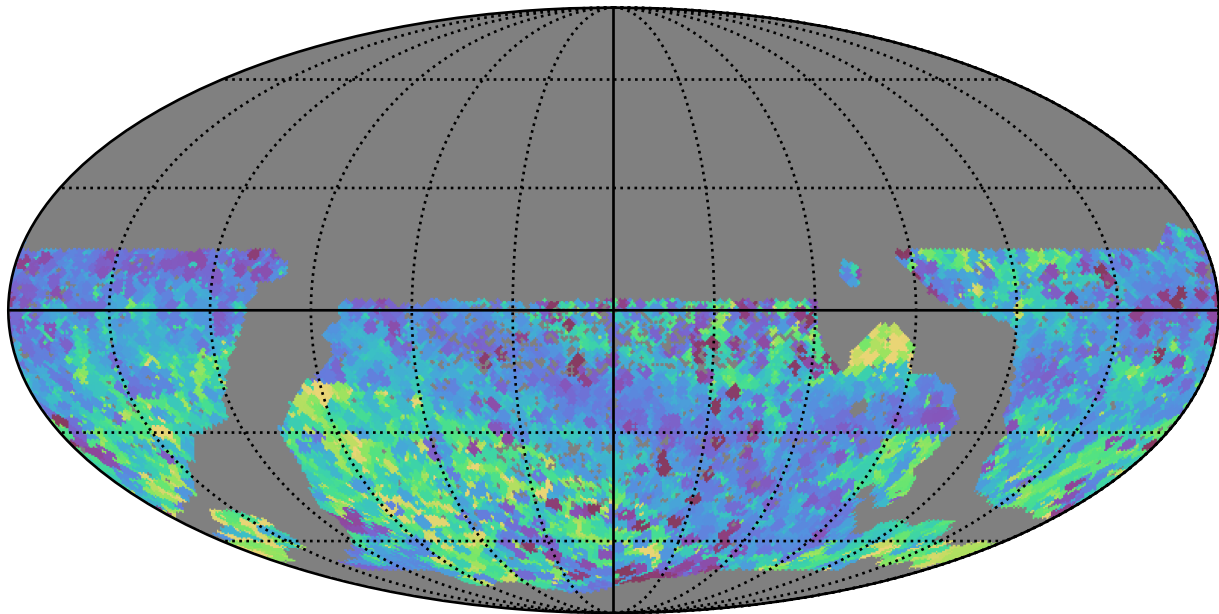
scp_reweight_v3.3_10yrs WFD all bands: Min skyBrightness
