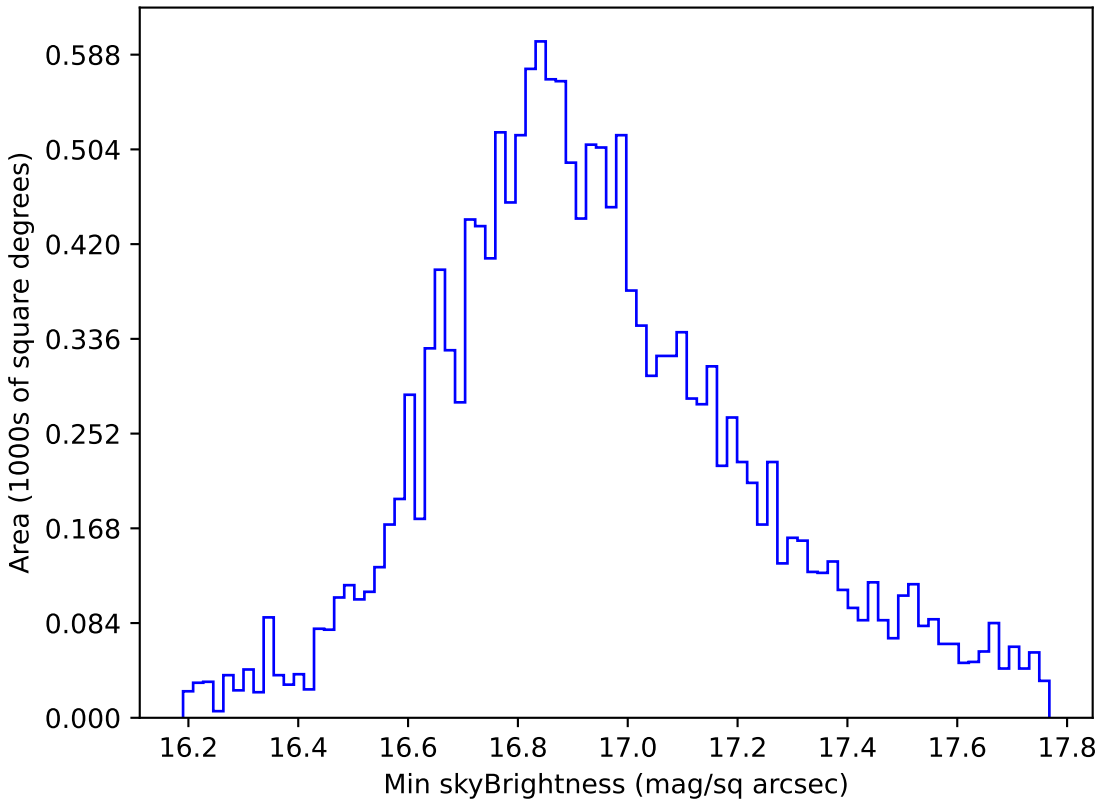
scp_reweight_v3.3_10yrs WFD all bands: Min skyBrightness
