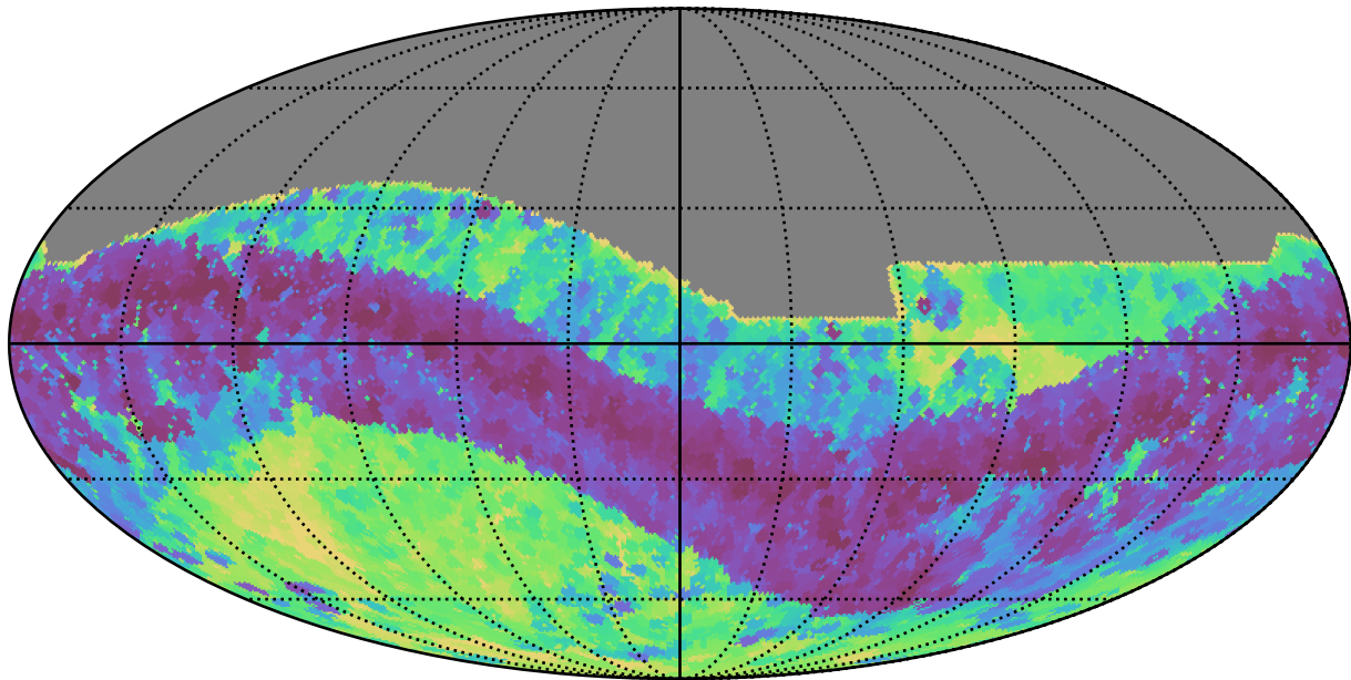
scp_reweight_v3.3_10yrs All sky z band: Min skyBrightness
