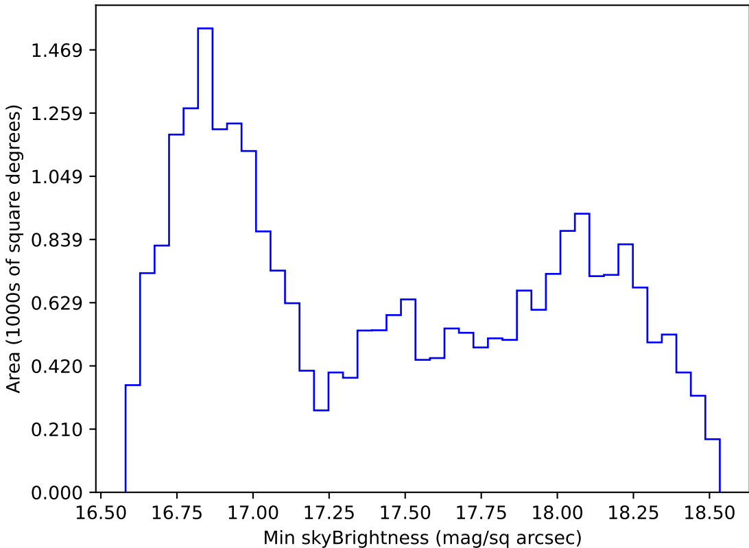
scp_reweight_v3.3_10yrs All sky z band: Min skyBrightness
