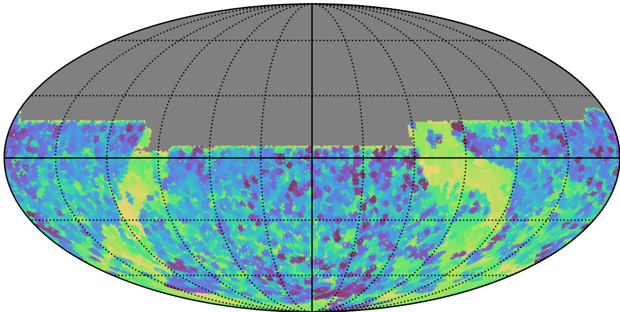
scp_reweight_v3.3_10yrs All sky y band: Min skyBrightness
