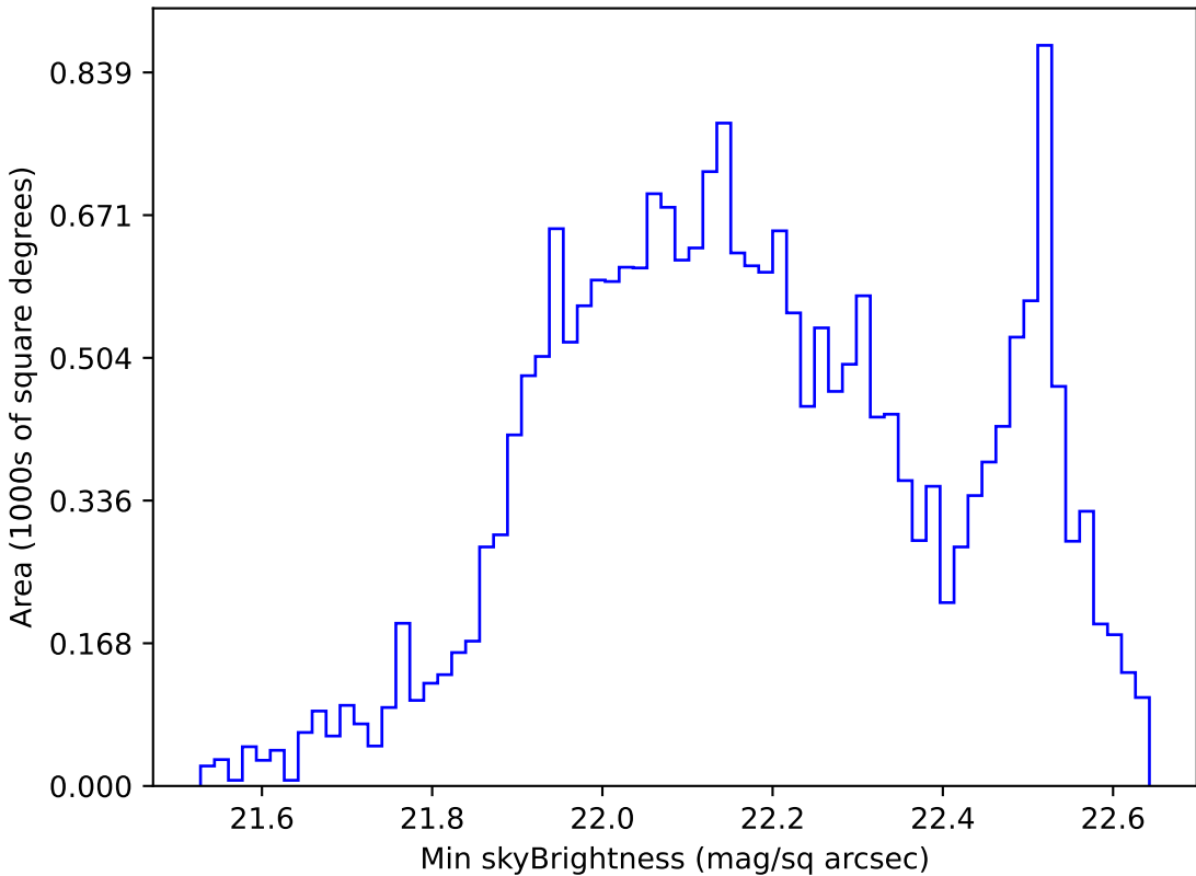
scp_reweight_v3.3_10yrs All sky u band: Min skyBrightness
