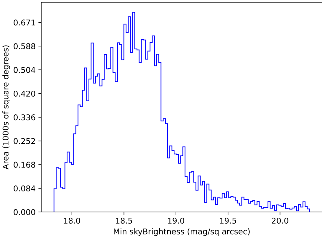
scp_reweight_v3.3_10yrs All sky r band: Min skyBrightness
