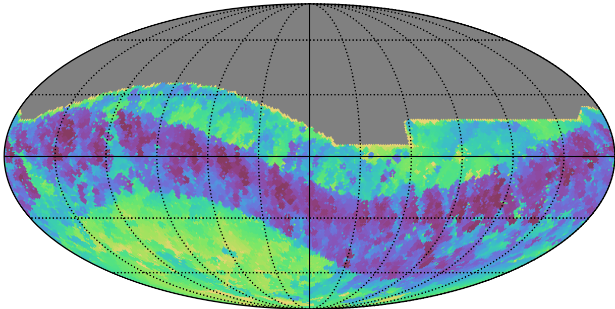
scp_reweight_v3.3_10yrs All sky i band: Min skyBrightness
