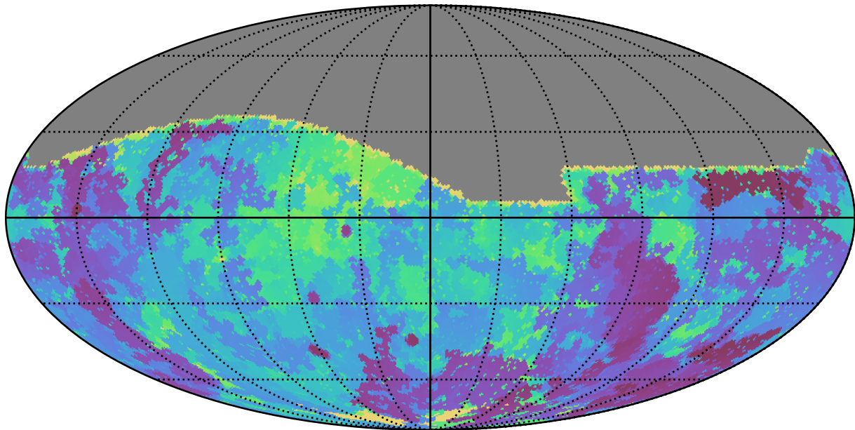
scp_reweight_v3.3_10yrs All sky g band: Min skyBrightness
