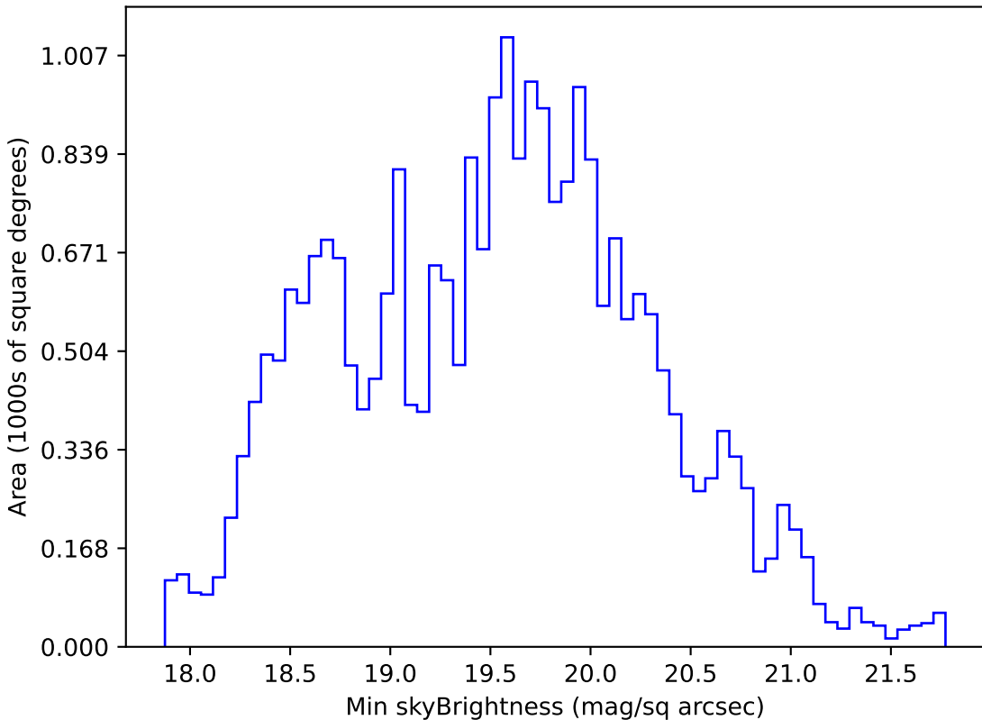
scp_reweight_v3.3_10yrs All sky g band: Min skyBrightness
