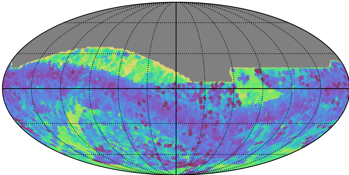
scp_reweight_v3.3_10yrs All sky all bands: Min skyBrightness
