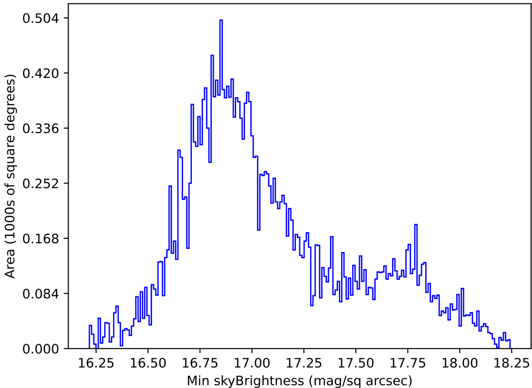
scp_reweight_v3.3_10yrs All sky all bands: Min skyBrightness
