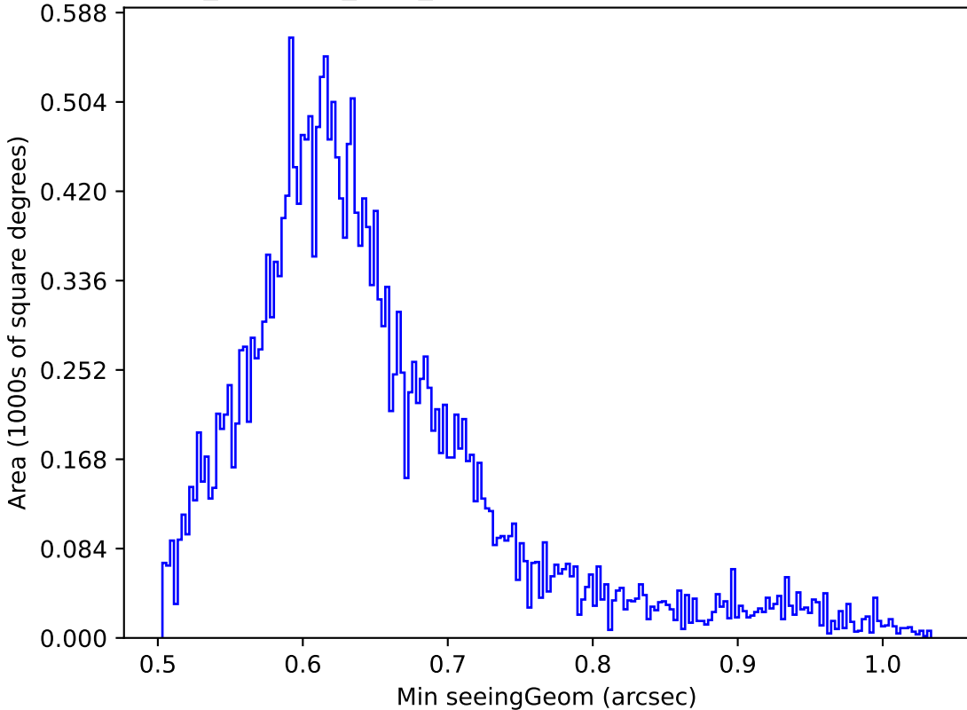
scp_reweight_v3.3_10yrs Yr 1 z band: Min seeingGeom
