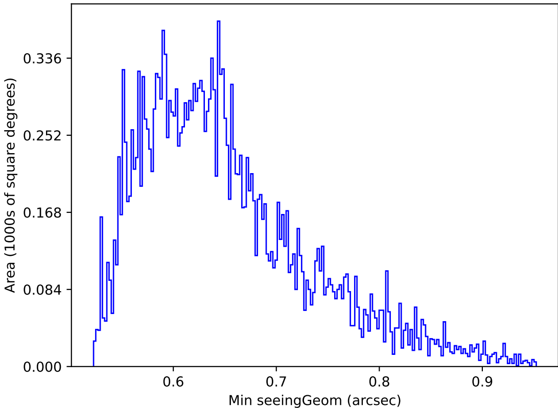
scp_reweight_v3.3_10yrs Yr 1 y band: Min seeingGeom
