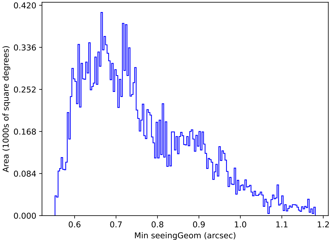
scp_reweight_v3.3_10yrs Yr 1 u band: Min seeingGeom
