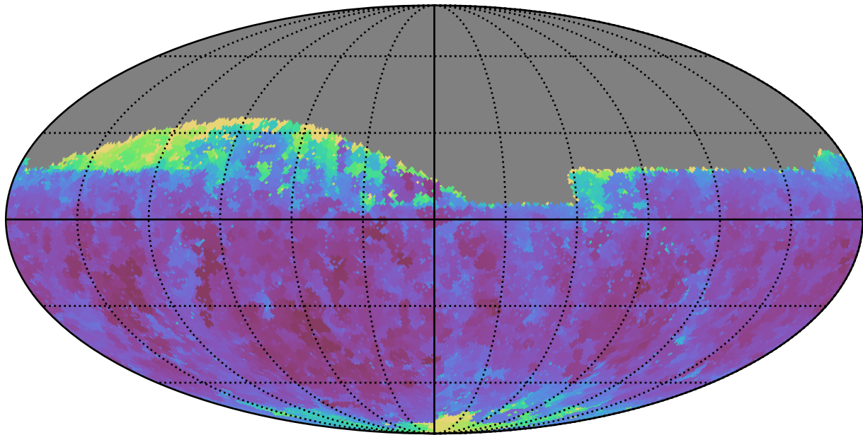
scp_reweight_v3.3_10yrs Yr 1 r band: Min seeingGeom
