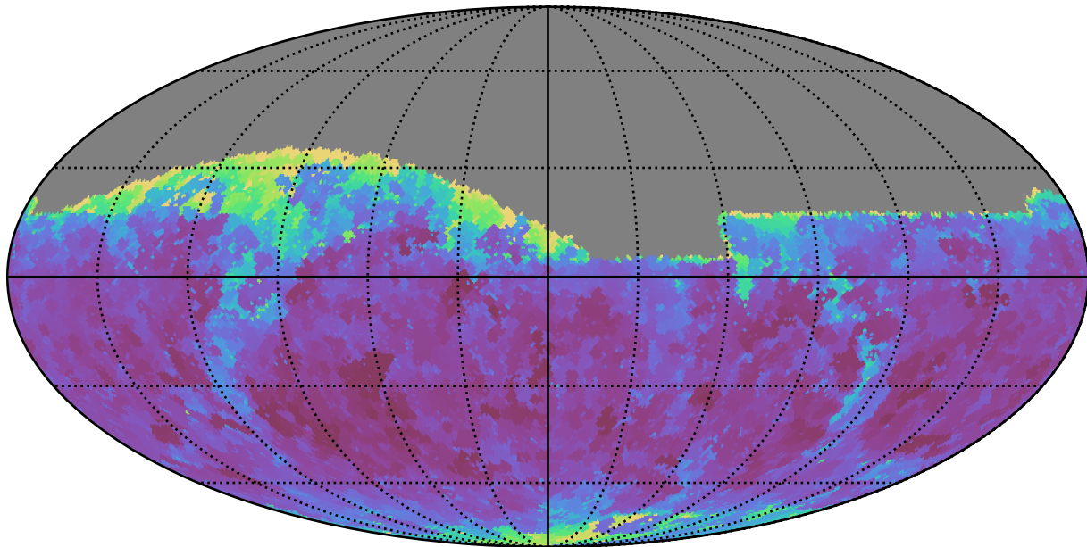
scp_reweight_v3.3_10yrs Yr 1 i band: Min seeingGeom
