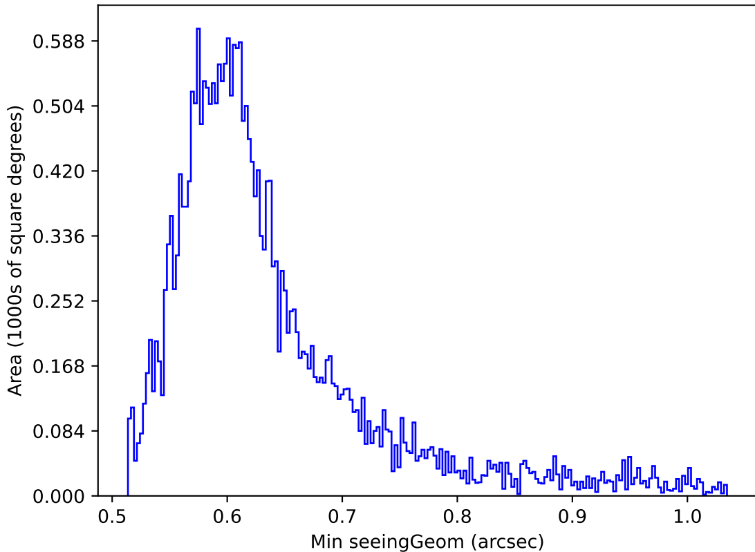
scp_reweight_v3.3_10yrs Yr 1 i band: Min seeingGeom
