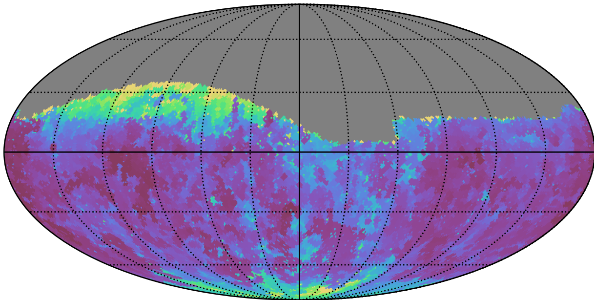
scp_reweight_v3.3_10yrs Yr 1 g band: Min seeingGeom
