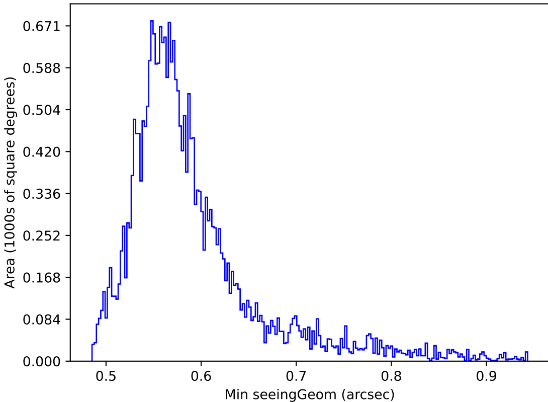
scp_reweight_v3.3_10yrs Yr 1 all bands: Min seeingGeom
