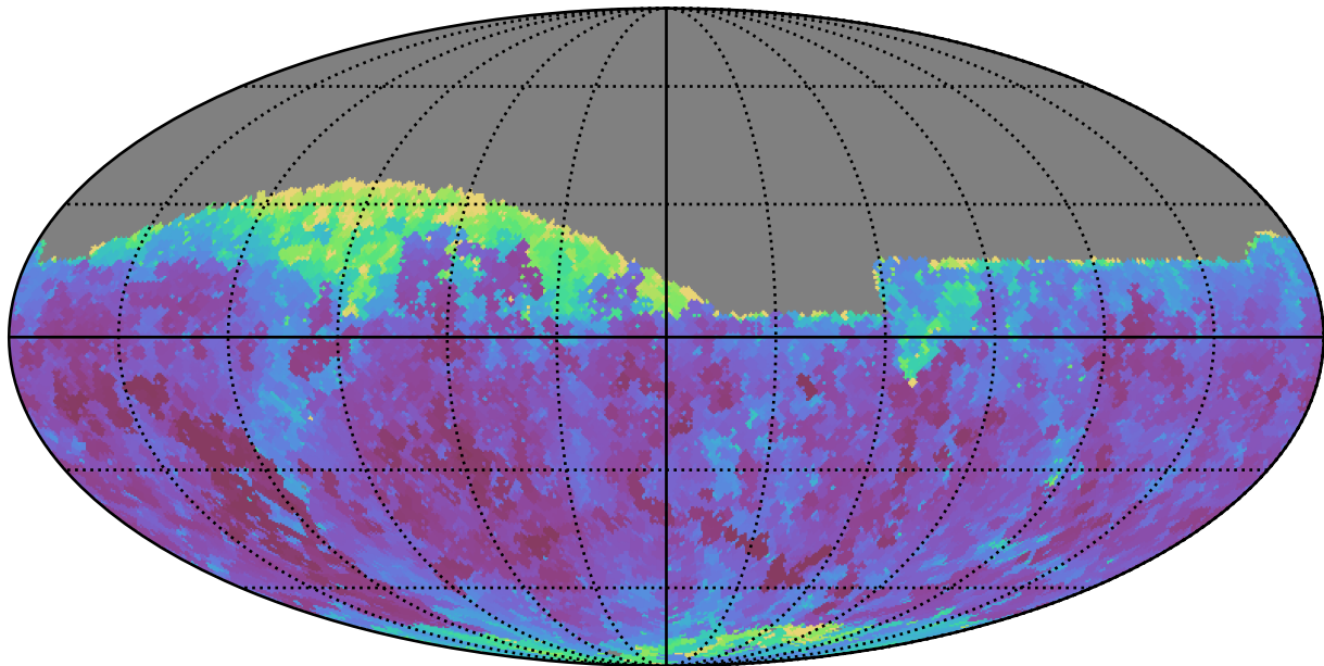
scp_reweight_v3.3_10yrs Yr 1 z band: Min seeingEff
