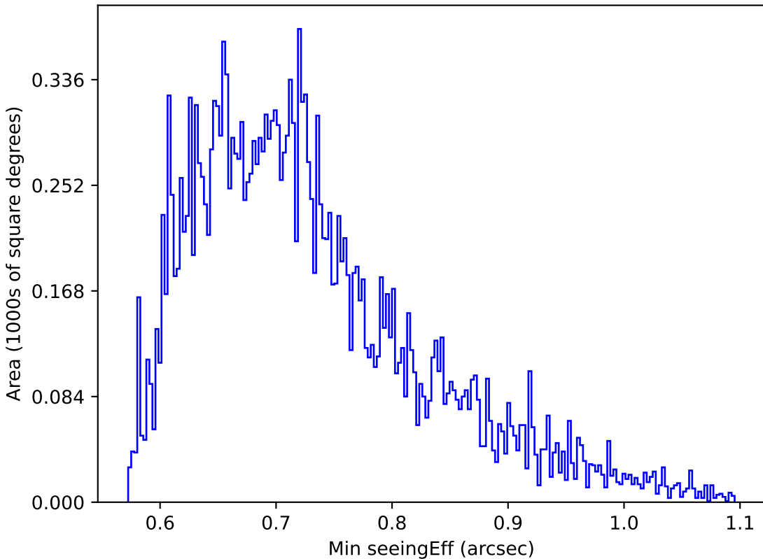
scp_reweight_v3.3_10yrs Yr 1 y band: Min seeingEff
