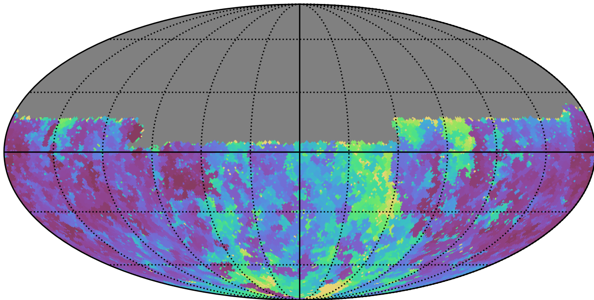
scp_reweight_v3.3_10yrs Yr 1 u band: Min seeingEff
