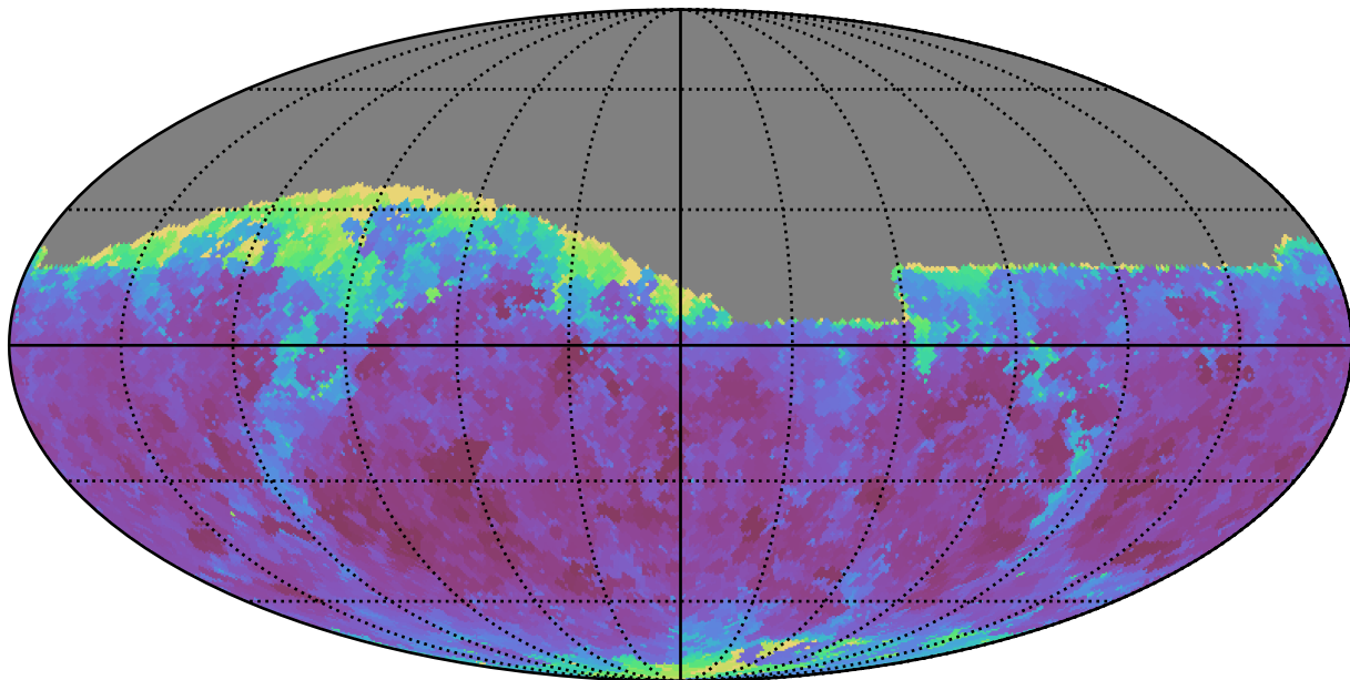
scp_reweight_v3.3_10yrs Yr 1 i band: Min seeingEff
