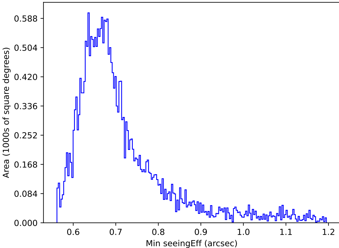
scp_reweight_v3.3_10yrs Yr 1 i band: Min seeingEff
