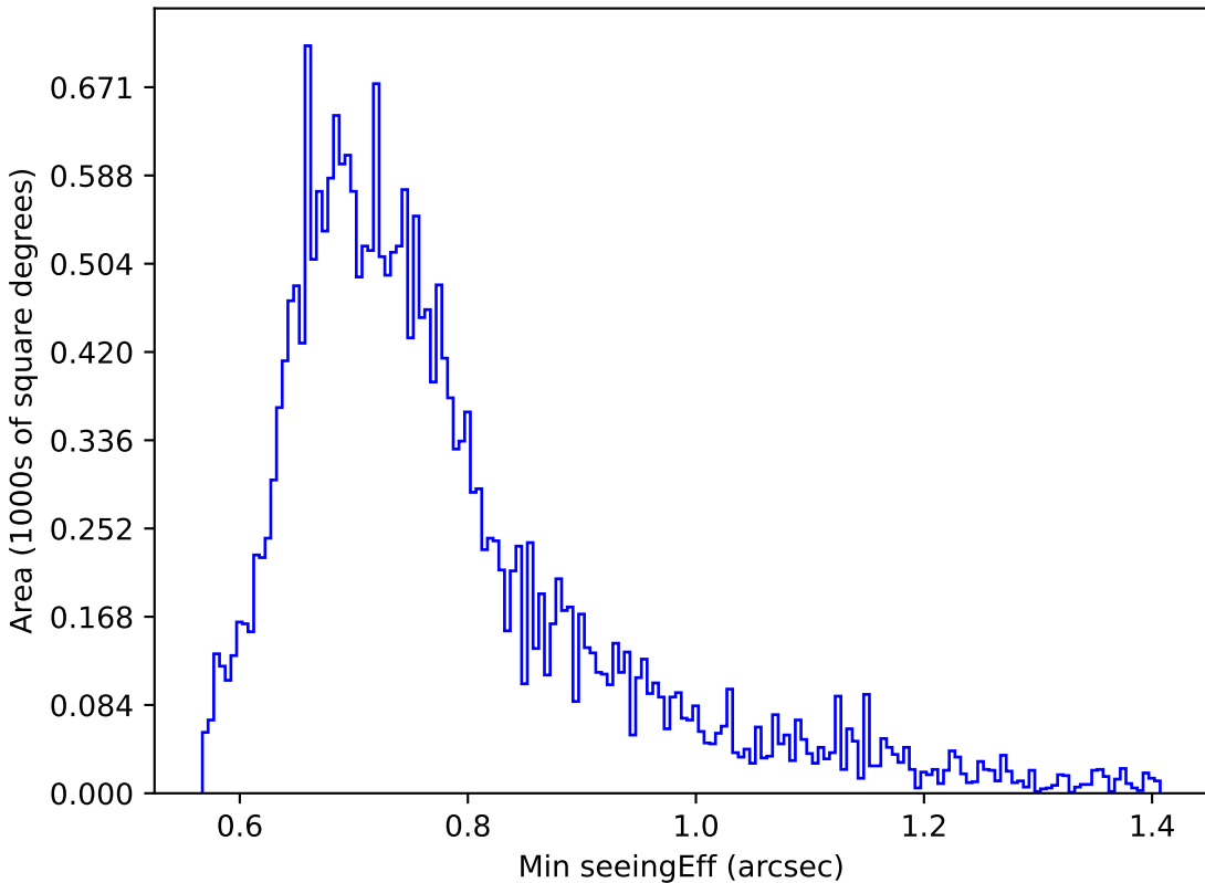
scp_reweight_v3.3_10yrs Yr 1 g band: Min seeingEff
