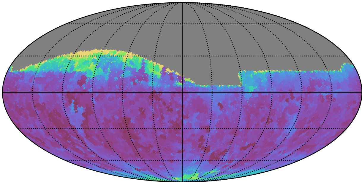
scp_reweight_v3.3_10yrs Yr 1 all bands: Min seeingEff
