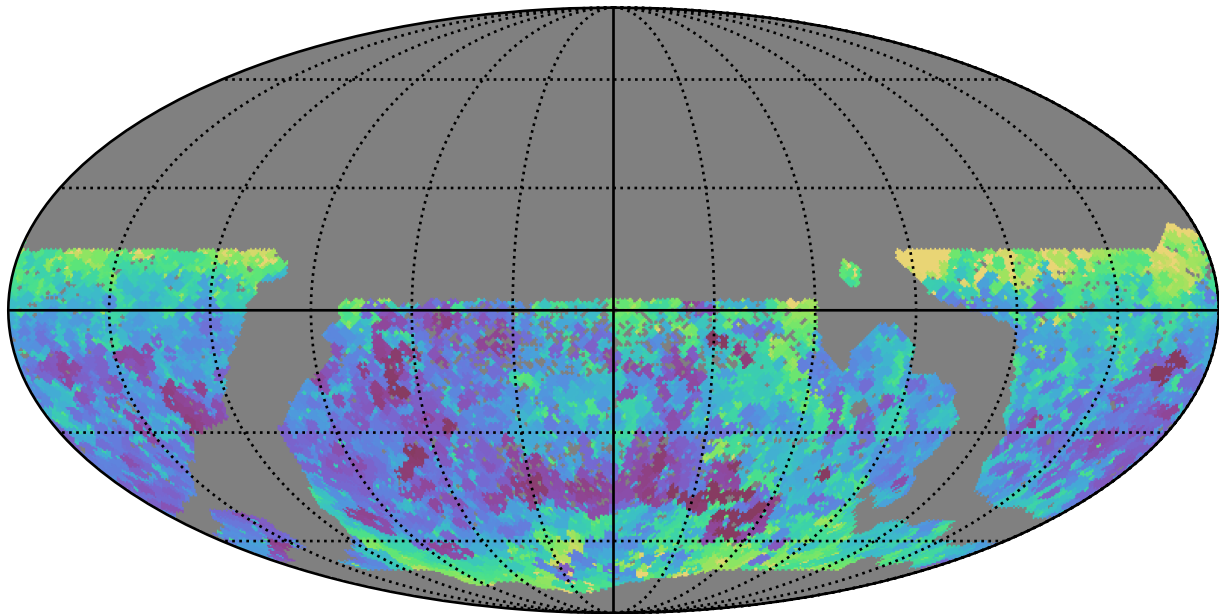
scp_reweight_v3.3_10yrs WFD z band: Min seeingEff
