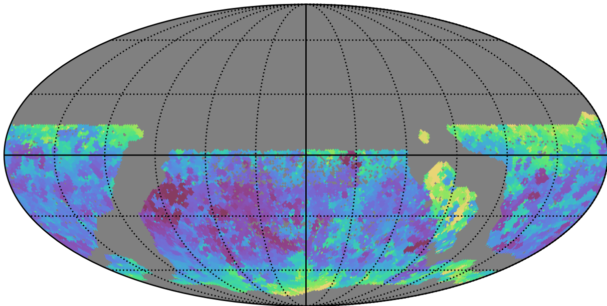
scp_reweight_v3.3_10yrs WFD y band: Min seeingEff
